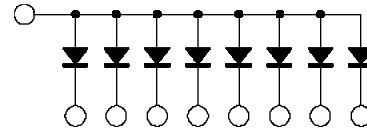
COMMON ANODE SG5770/SG6507
