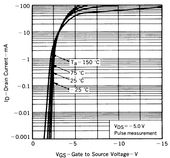
TRANSFER CHARACTERISTICS
