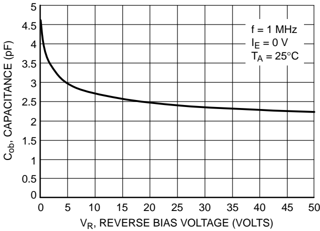
Figure 64. Output Capacitance
