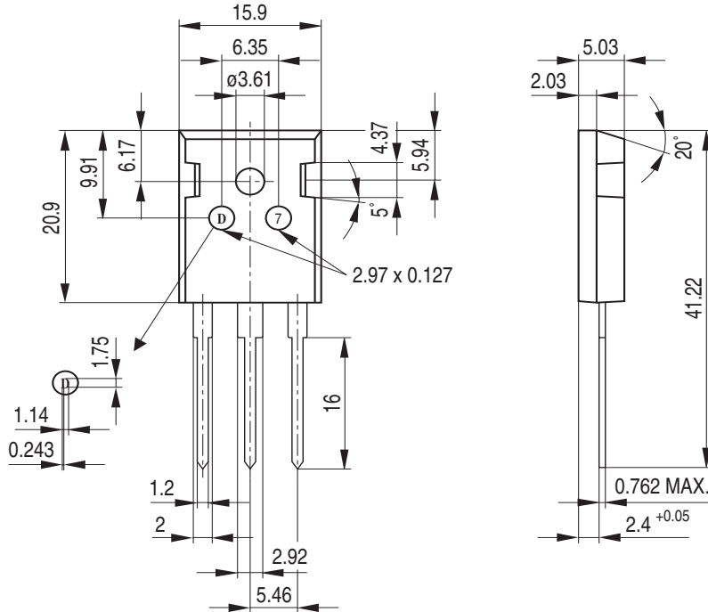
P-TO-247-3-1
