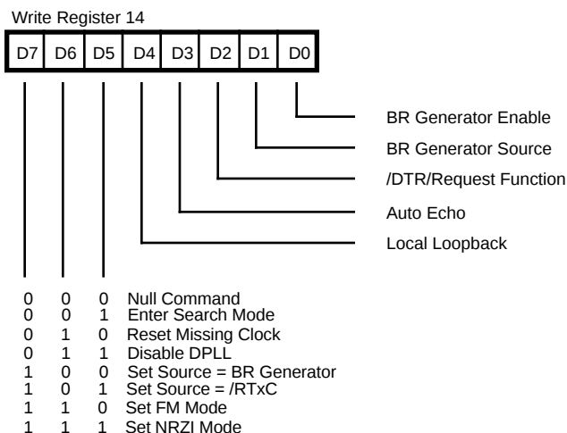
Figure 5-17. Write Register 14
