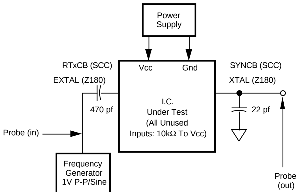
Figure 6. Gain Measurement
