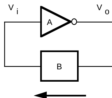
Figure 1. Basic Circuit and Loop Gain
