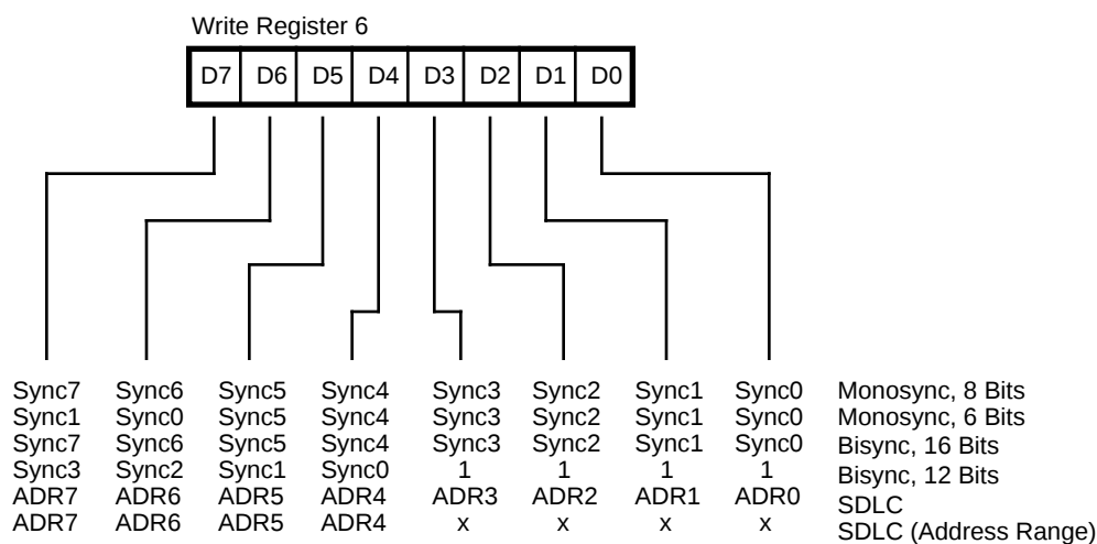
Figure 5-8. Write Register 6
