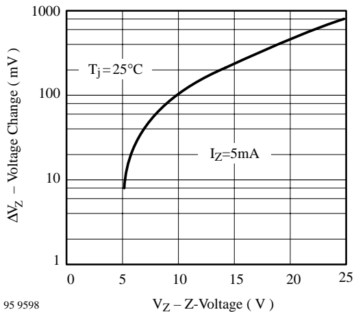
Typical Change of Working Voltage under Operating Conditions at T_{amb}=25^\circ\text{C}
