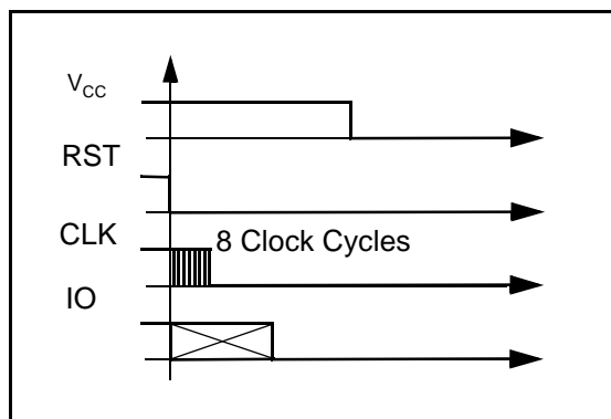
Figure 18. SCI Deactivation Sequence after a Card Extraction
