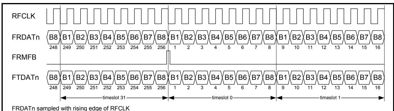
Figure 26 Framer Interface in SYM2 E1
