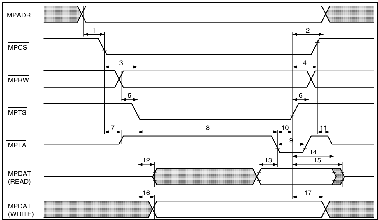
Figure 70 Motorola Mode Timing Diagram
