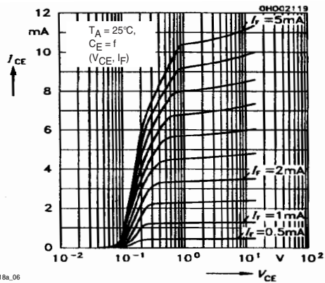
Fig. 8 Output Characteristics
