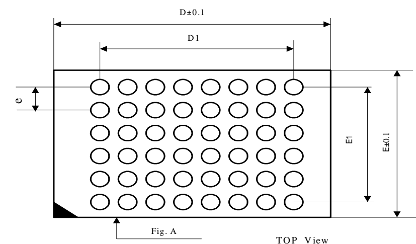
48 Mini-BGA 6*8mm
