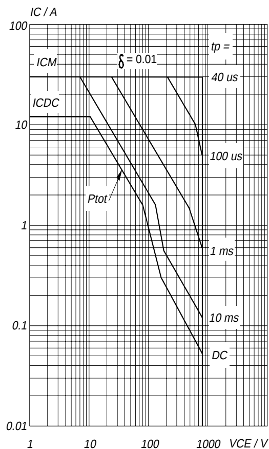
Fig.15. Forward bias safe operating area. T_{mb} = 25^\circ\text{C} I_{CDC} & I_{CM} = f(V_{CE}) ; I_{CM} single pulse; parameter t_p Second-breakdown limits independent of temperature.
