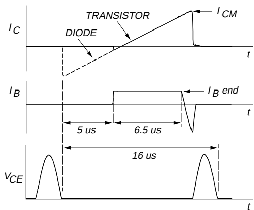
Fig.3. Switching times waveforms.
