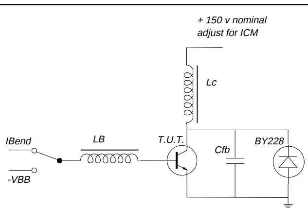
Fig.5. Switching times test circuit.
