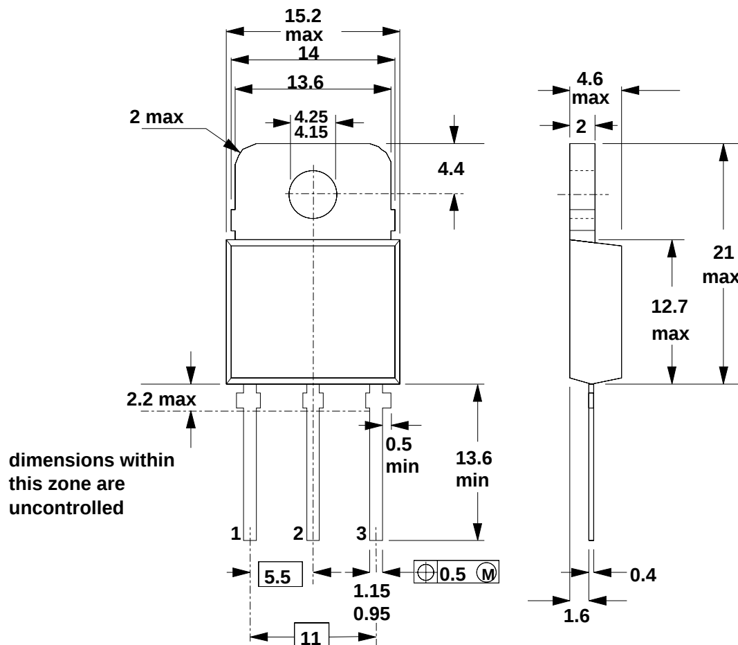
Fig.17. SOT93; pin 2 connected to mounting base.
