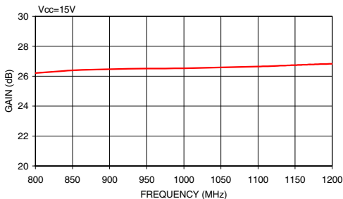
TO-0812LN GAIN
