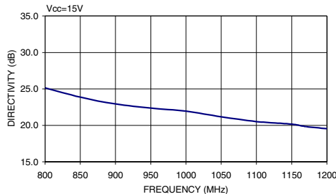
TO-0812LN DIRECTIVITY
