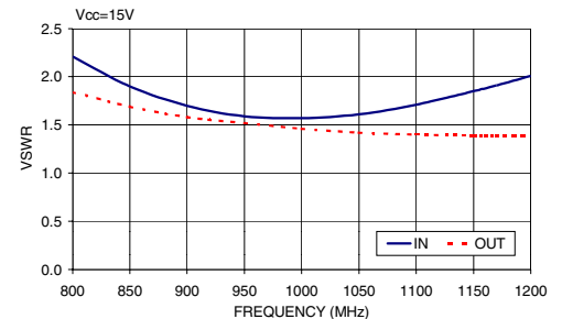
TO-0812LN VSWR
