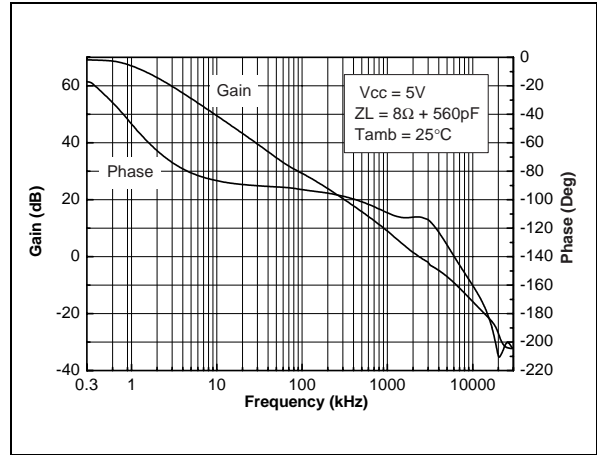
Fig. 2 : Open Loop Frequency Response
