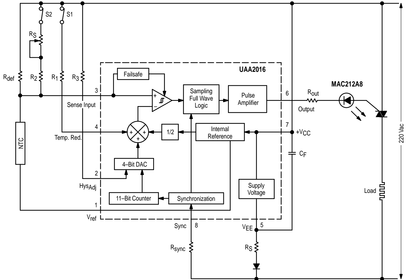
Figure 1. Application Schematic
