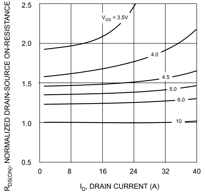
Fig. 2, On-Resistance vs Gate Voltage and Drain Current
