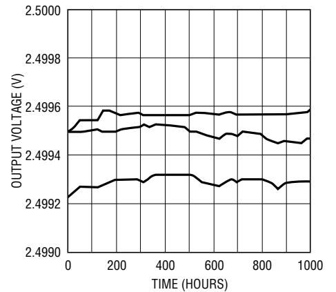
Long-Term Drift Three Typical Parts (S8 Package)
