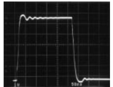
Large-Signal Transient ( A_V = -1 , C_L = 200pF )
