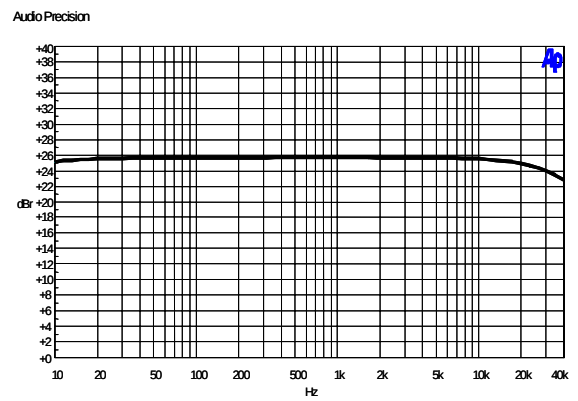
Figure 12. Frequency Response
