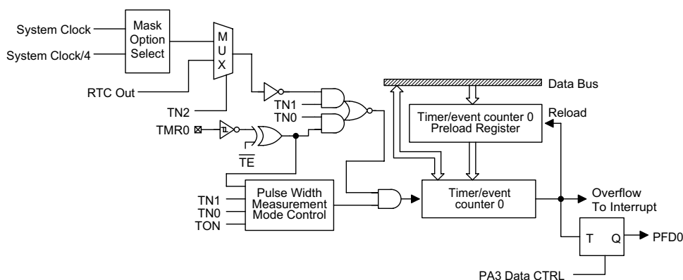
Timer/event counter 1
