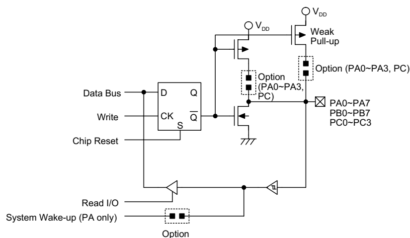
Input/output ports
