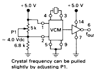
FIGURE 3 — VOLTAGE-CONTROLLED MULTIVIBRATOR
