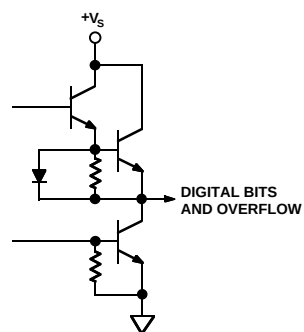
AD9020 Equivalent Digital Outputs
