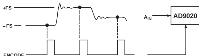
Imaging Application Using AD9020
