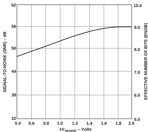
AD9020 SNR and ENOB vs. Reference Voltage
