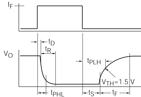
Figure 6. Switching timing
