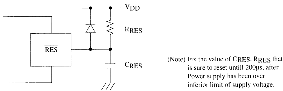
Figure4. Reset circuit
