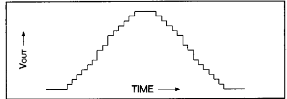
Fig. 2 Typical Sine Wave Output-Column Tones
