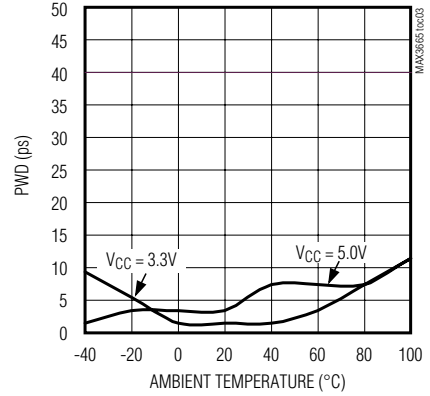
PULSE-WIDTH DISTORTION vs. TEMPERATURE (INPUT = 450 \mu A p-p )
