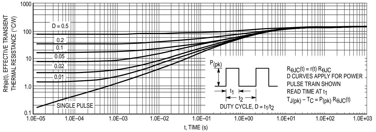
Figure 15. Thermal Response
