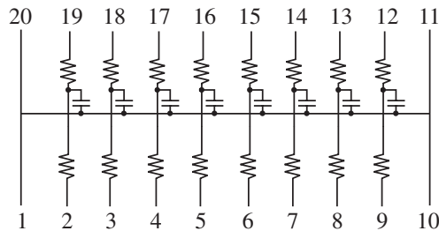
SCHEMATIC CONFIGURATION
