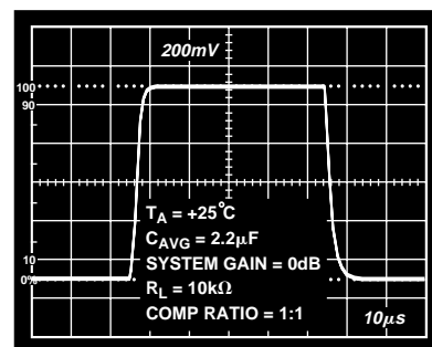
Figure 12. Large Signal Transient Response
