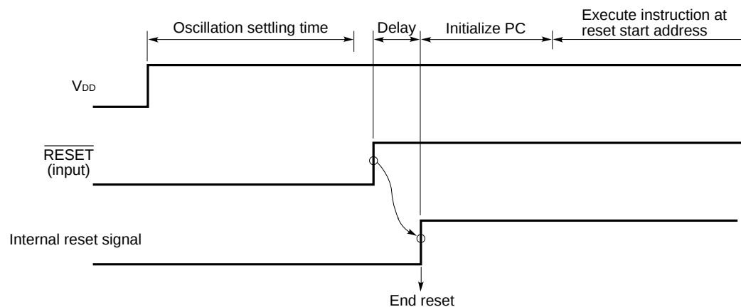
Fig. 12-2 Power-On Reset
