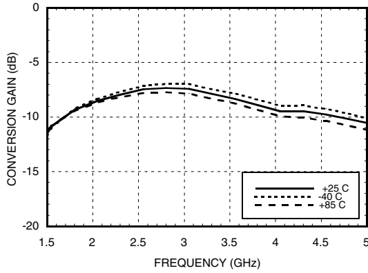
Conversion Gain vs Temperature @ LO = +13 dBm
