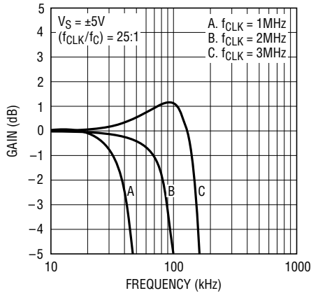
Passband Gain vs f_{CLK} at 85°C
