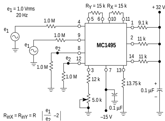
Figure 7. Input Resistance
