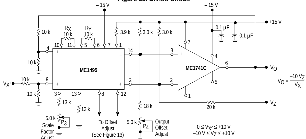
Figure 25. Divide Circuit
