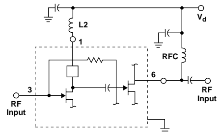
Figure 18. Interstage Inductor L2 and Bias Current.
