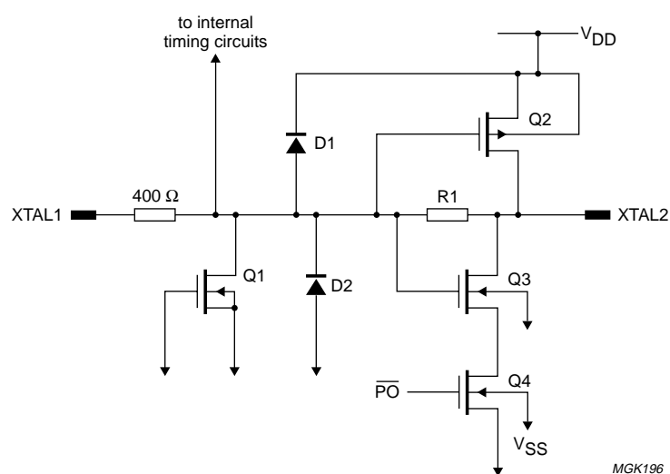
Fig.18 P89C738/P89C739 oscillator internal circuit.
