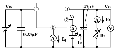
Fig.1 Test Circuit
