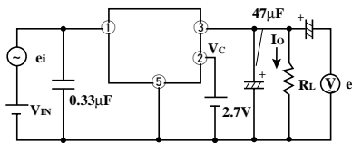
Fig.2 Test Circuit for Ripple Rejection
