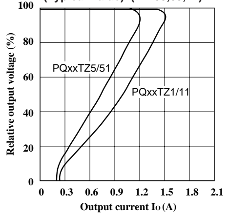
Fig.4 Overcurrent Protection Characteristics (Typical Value) (xx=05,09,12)
