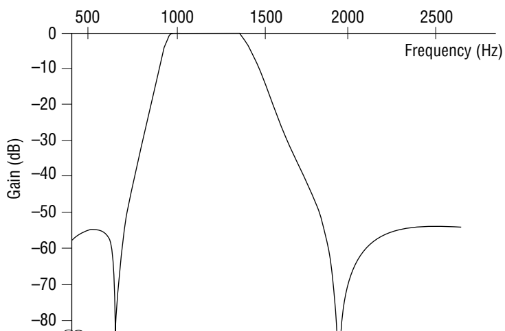
Figure 5 MSM6946 Low Band Filter
