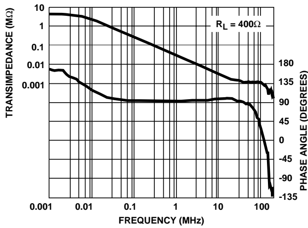
FIGURE 40. TRANSIMPEDANCE vs FREQUENCY
