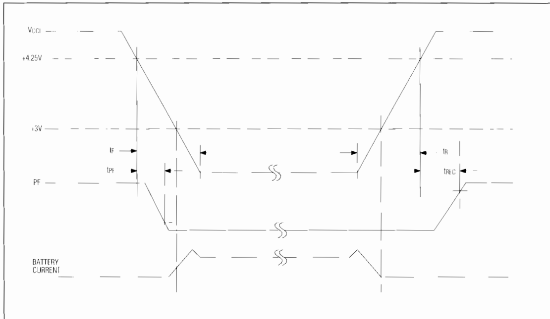
Figure 1. Power-Down/Power-Up Conditions
