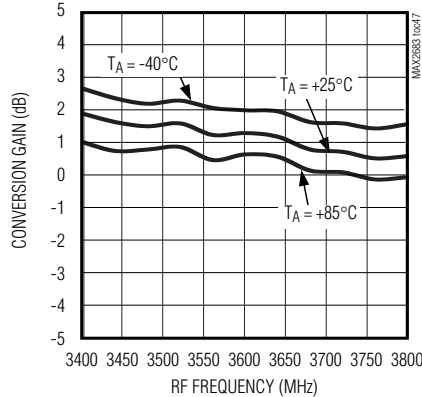
CONVERSION GAIN vs. RF FREQUENCY (ENX2 = VCC)
