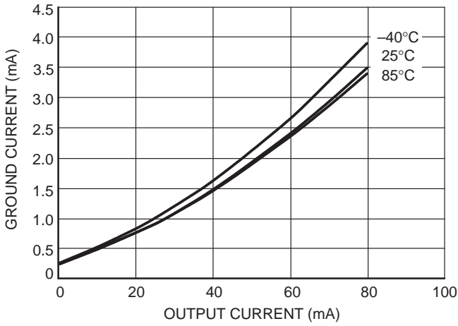
Figure 1. Ground Current versus Output Current
