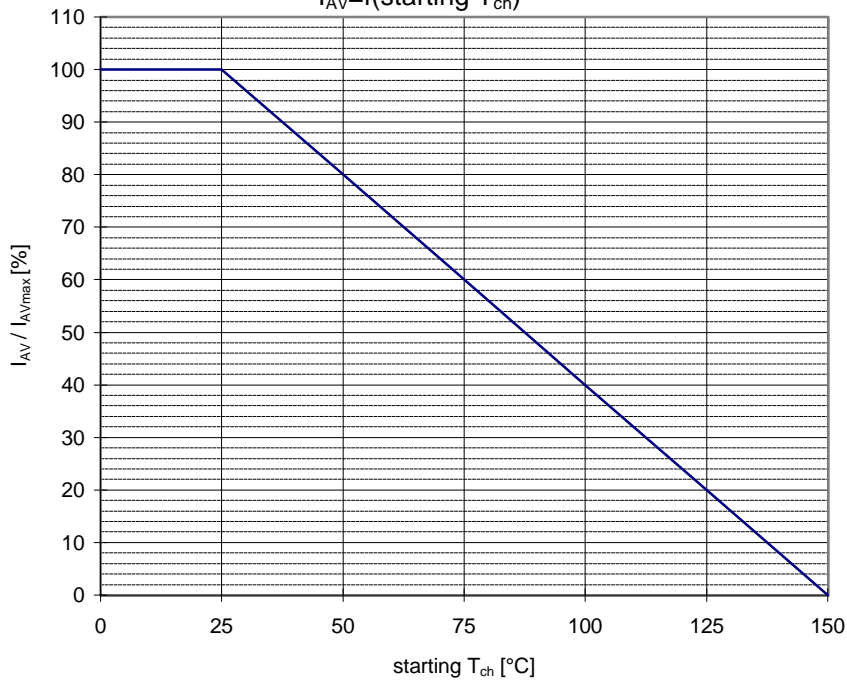
Maximum Avalanche Current vs. starting T_{ch} I_{AV}=f(\text{starting } T_{ch})
