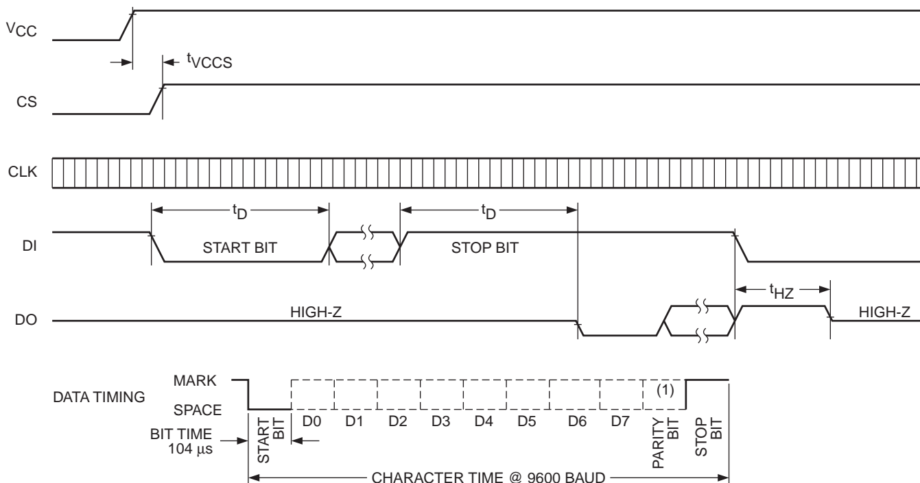
Figure 1. A.C. Timing
