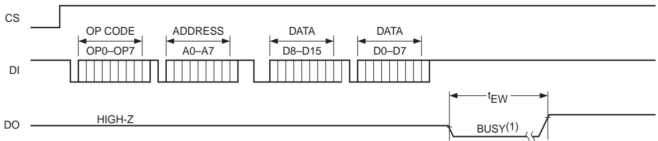
Figure 5. Program/Erase Timing (x16 Format)
