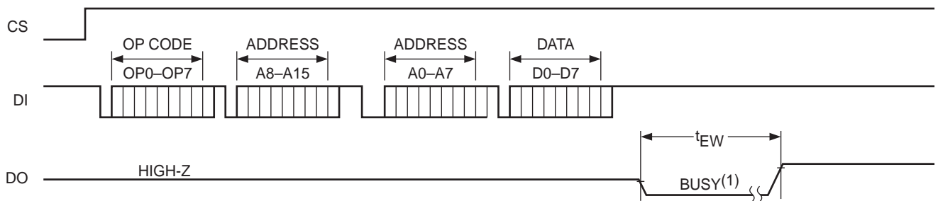
Figure 4. Program/Erase Timing (x8 Format)
