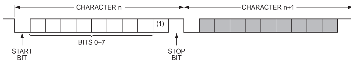
Figure 13. Asynchronous Communication Protocol
