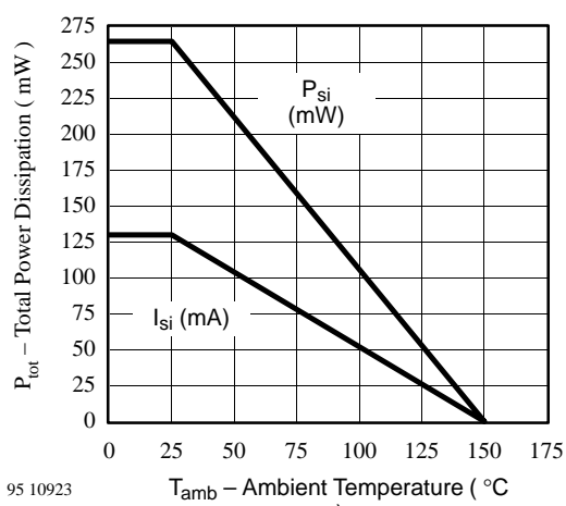
Figure 1. Derating diagram
