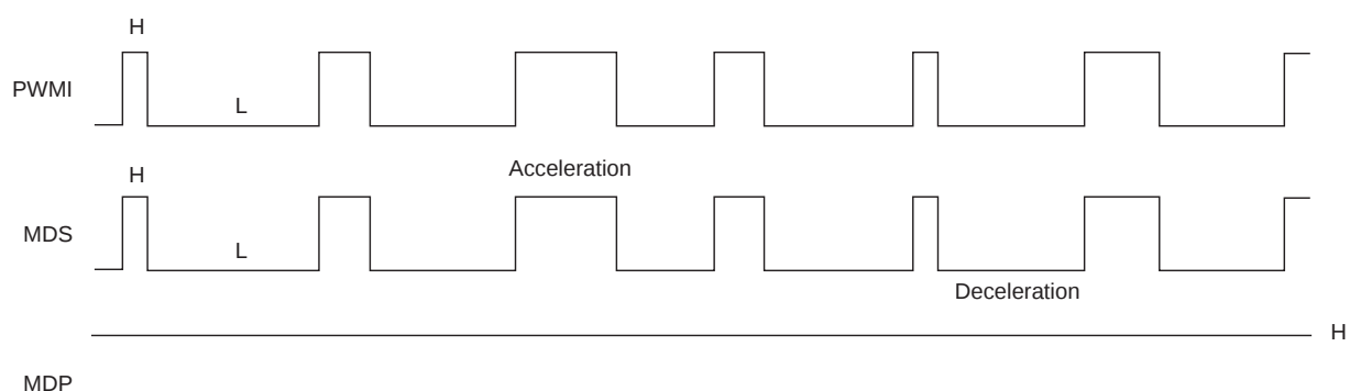
Timing Chart 1-29
