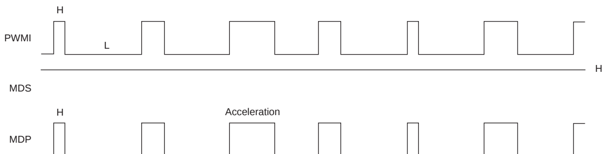
Timing Chart 1-29
