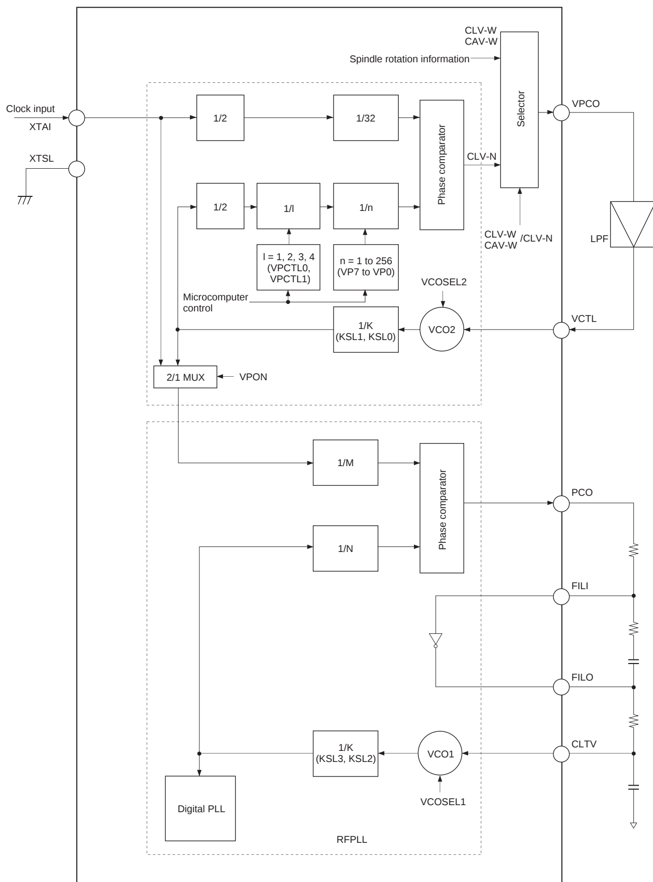
Block Diagram 4-1
