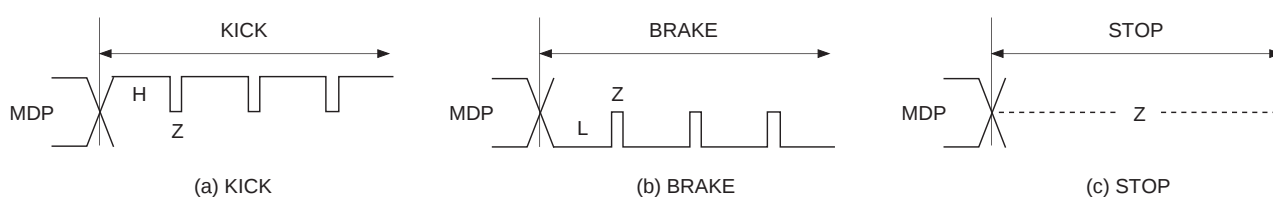
Timing Chart 1-8
