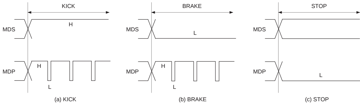
Timing Chart 1-19
