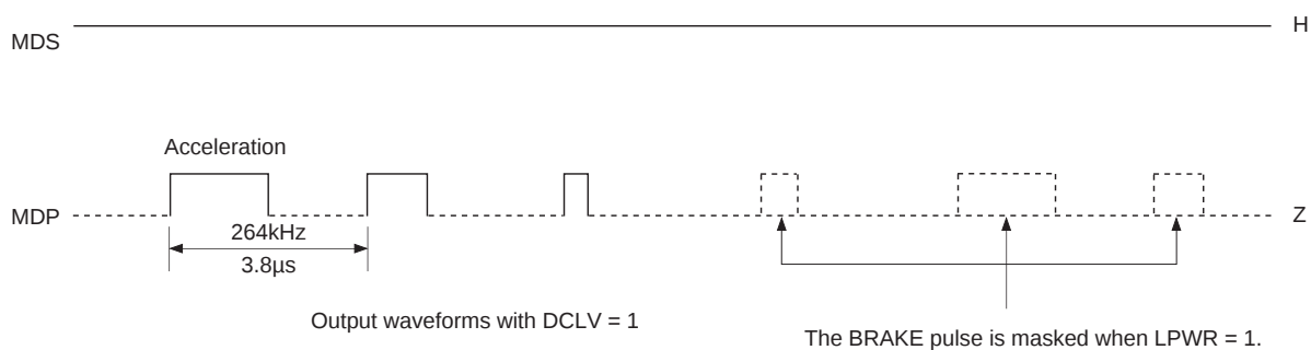
Timing Chart 1-36
