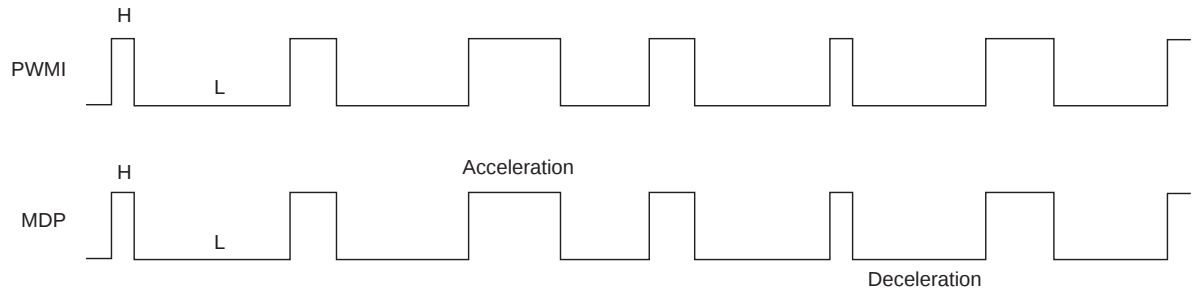
Timing Chart 1-17
