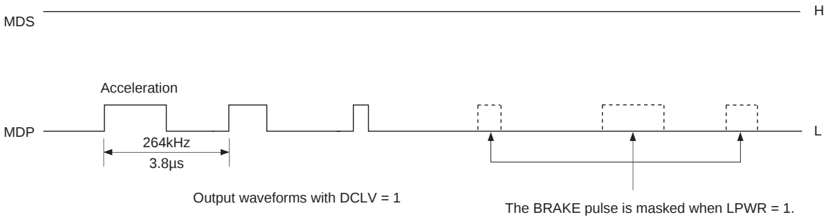
Timing Chart 1-26
