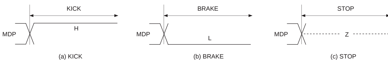
Timing Chart 1-10
