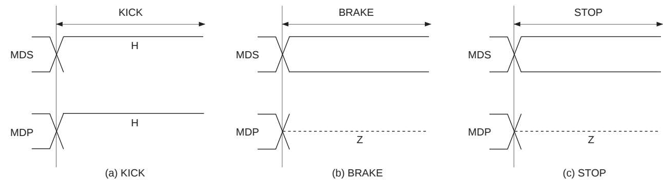
Timing Chart 1-33
