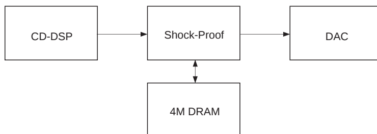
PCM Data Flow (Example for 4M \times 1 mode)
