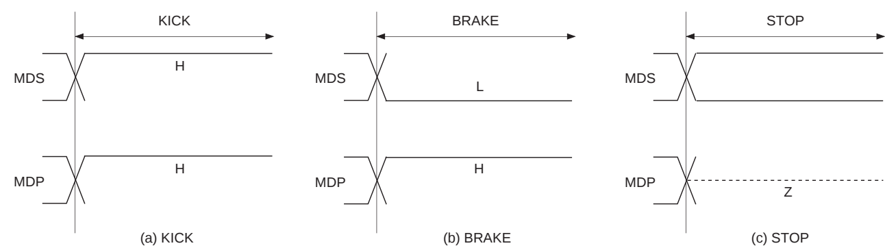
Timing Chart 1-33
