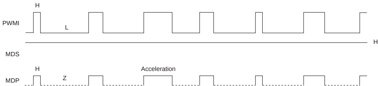
Timing Chart 1-39
