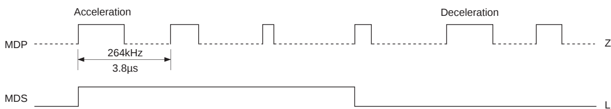
Timing Chart 1-36
