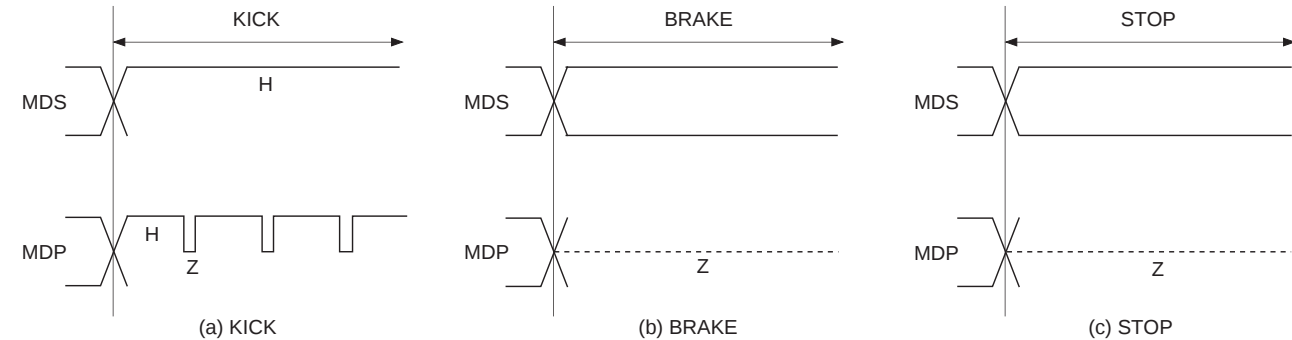
Timing Chart 1-32
