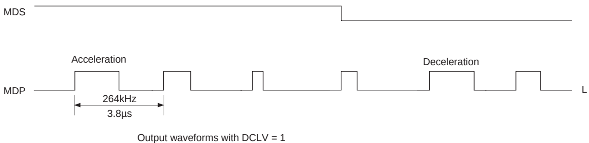
Timing Chart 1-25
