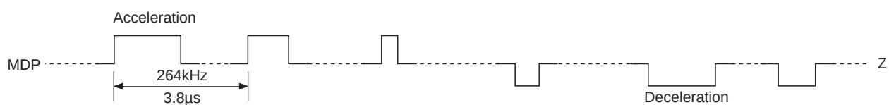
Timing Chart 1-14
