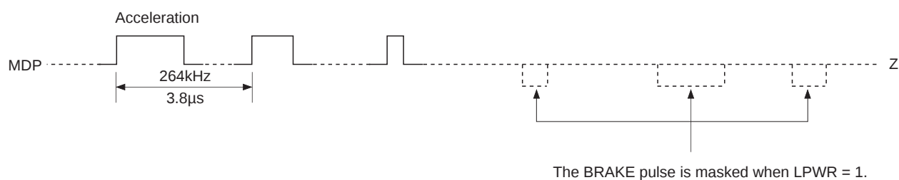
Timing Chart 1-15
