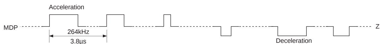
Timing Chart 1-12
