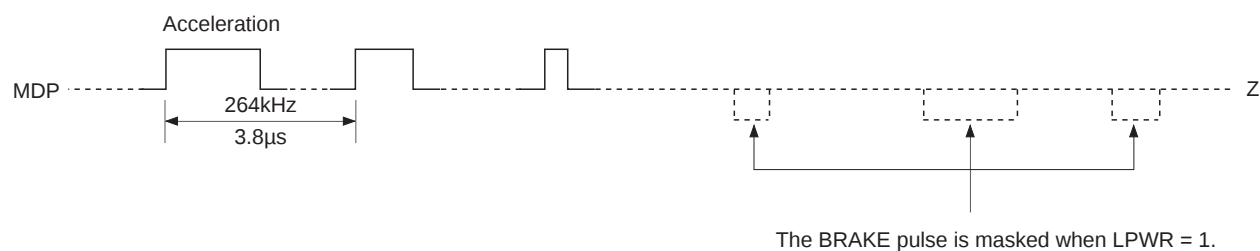
Timing Chart 1-14
