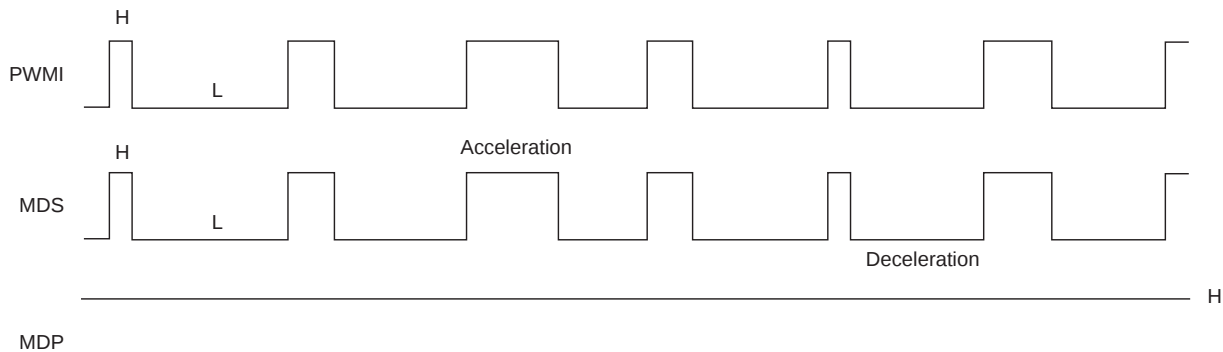
Timing Chart 1-39
