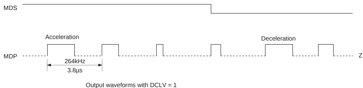
Timing Chart 1-35
