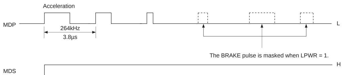
Timing Chart 1-28
