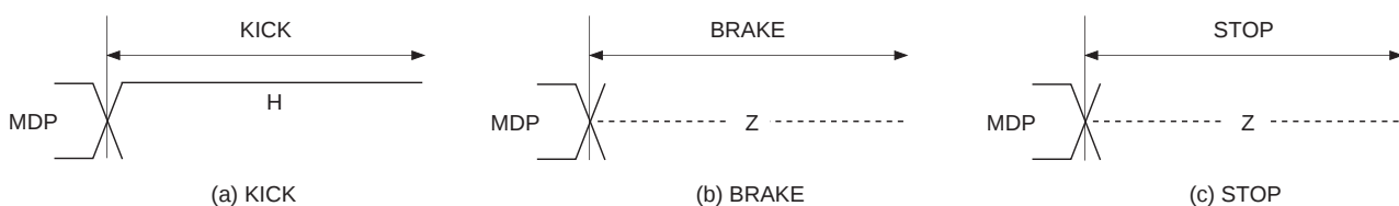
Timing Chart 1-10
