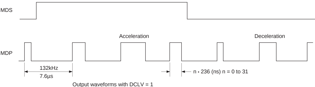
Timing Chart 1-24
