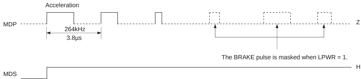
Timing Chart 1-38
