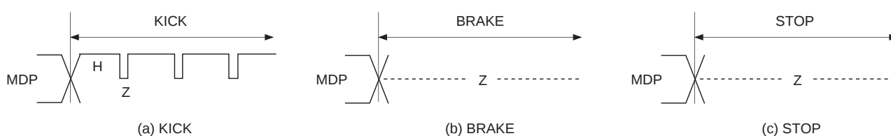
Timing Chart 1-9
