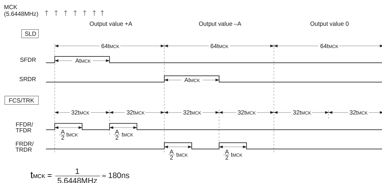
Timing Chart 5-20.
