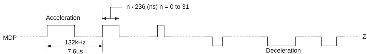
Timing Chart 1-11
