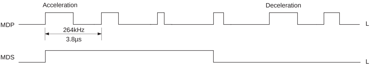
Timing Chart 1-26
