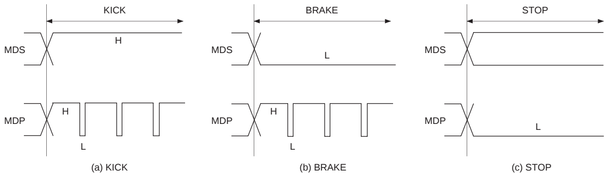
Timing Chart 1-19
