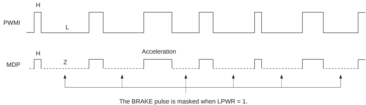
Timing Chart 1-17
