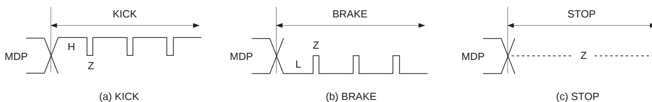
Timing Chart 1-7
