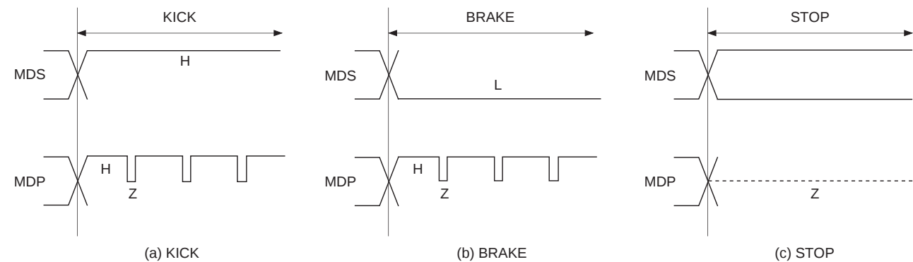
Timing Chart 1-31
