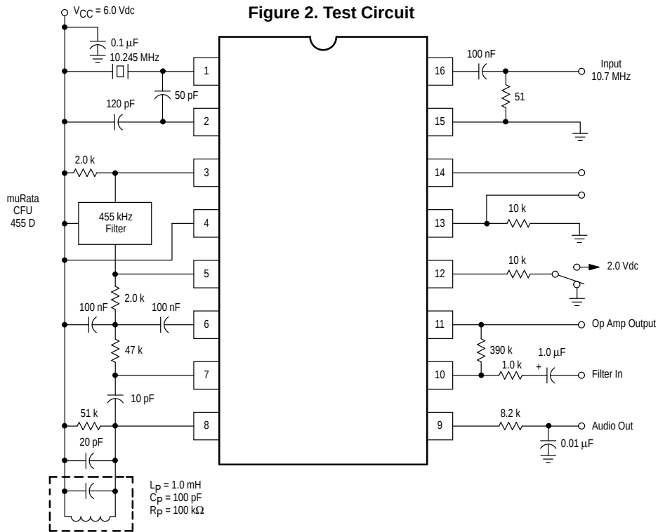
Figure 2. Test Circuit
