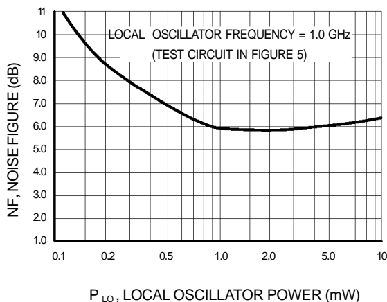
Figure 4. Noise Figure
