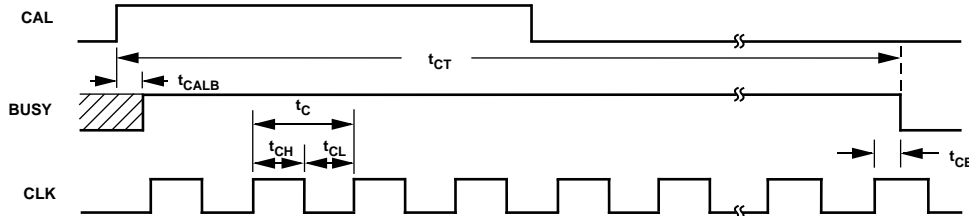
Figure 1. AD1876 Calibration Timing
