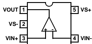
EL5111 (5-PIN TSOT) TOP VIEW
