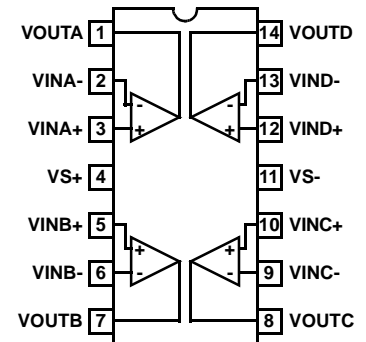
EL5411 (14-PIN TSSOP, HTSSOP) TOP VIEW
