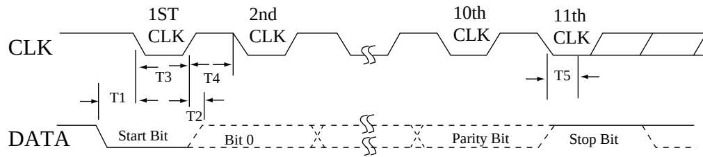
Fig 3. Keyboard output data timings
